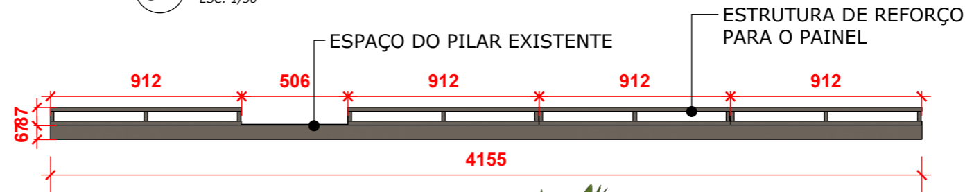
02 PAINEL GALERIA | FRONTAL ESC: 1/30
