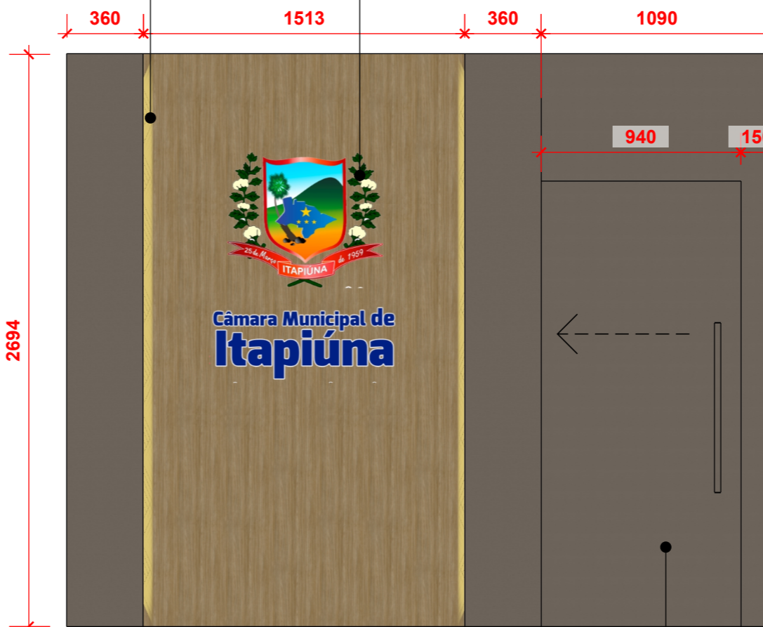
03 PAINEL E PORTA | FRONTAL ESC: 1/25
